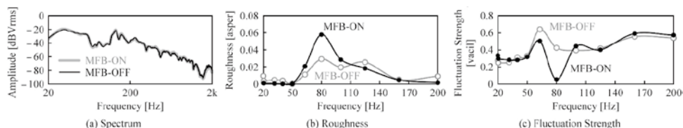
Fig.1 Frequency spectrum and psychoacoustic parameters of sound reproduced by sub-woofer with motional feedback system (MFB).
